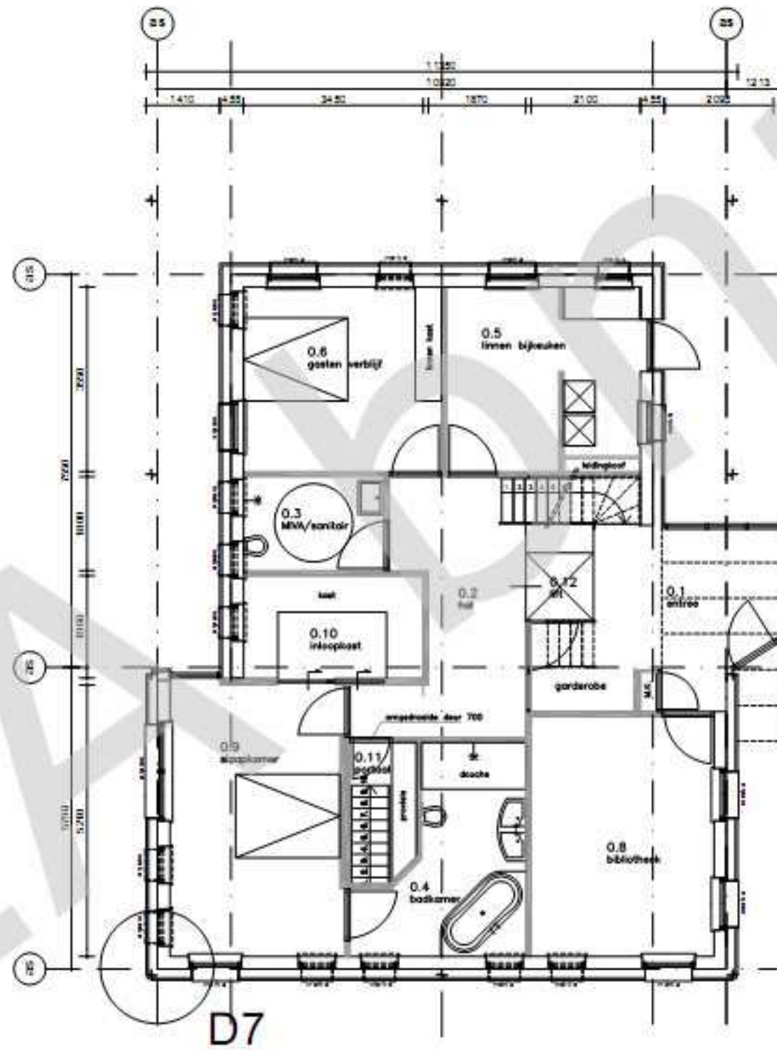
beganegrand
